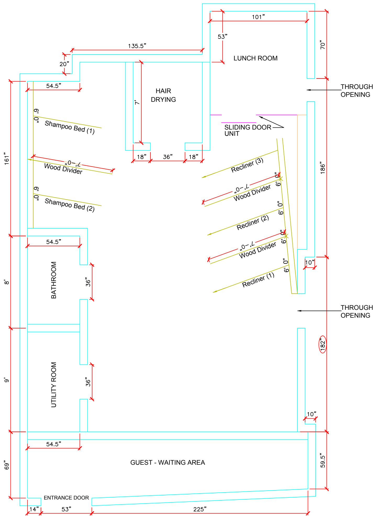
FLOOR PLAN UNIT 107 SCALE 1/4" = 1'-0"
