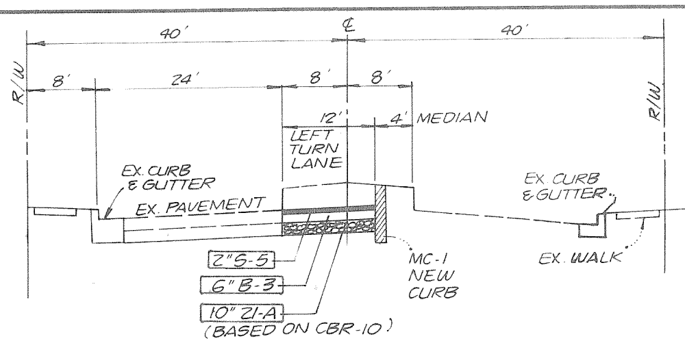
HERNDON PARKWAY (TS-2) STREET SECTION STATION 4+50 TO 6+32 NO SCALE
