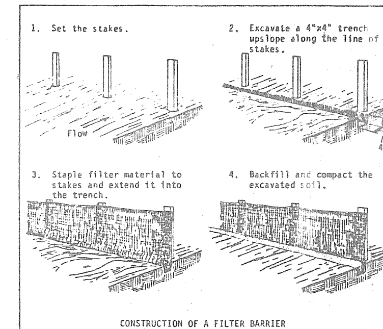
CONSTRUCTION OF A FILTER BARRIER Source: Installation of Straw and Fabric Filter Barriers Plate 1.06a for Sediment Control, Sherwood and Wynn
