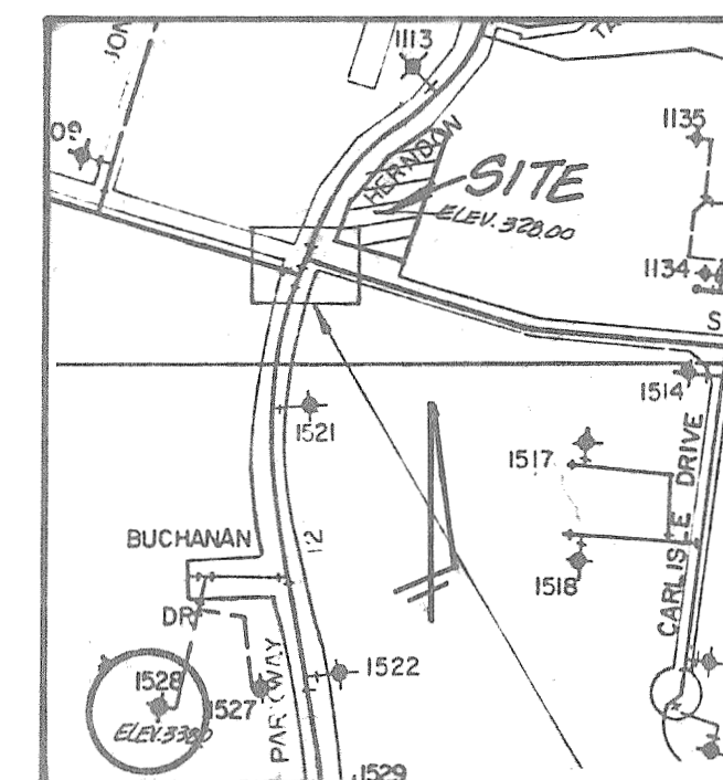
WATER LINE VICINITY MAP
