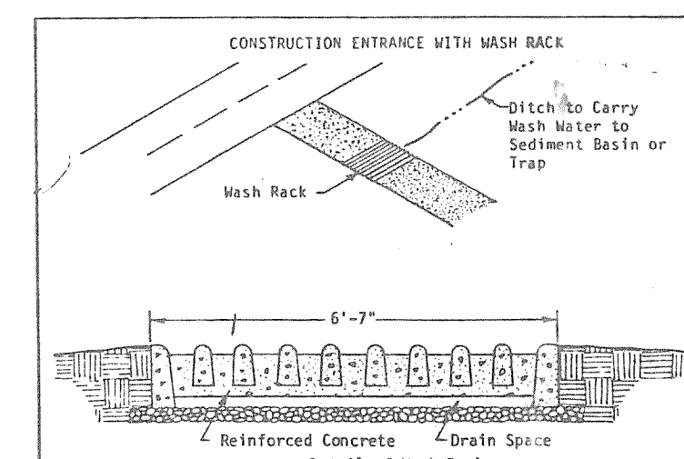
CONSTRUCTION ENTRANCE WITH WASH RACK Source: Smith Cottagegard Company Plate 1.01b
