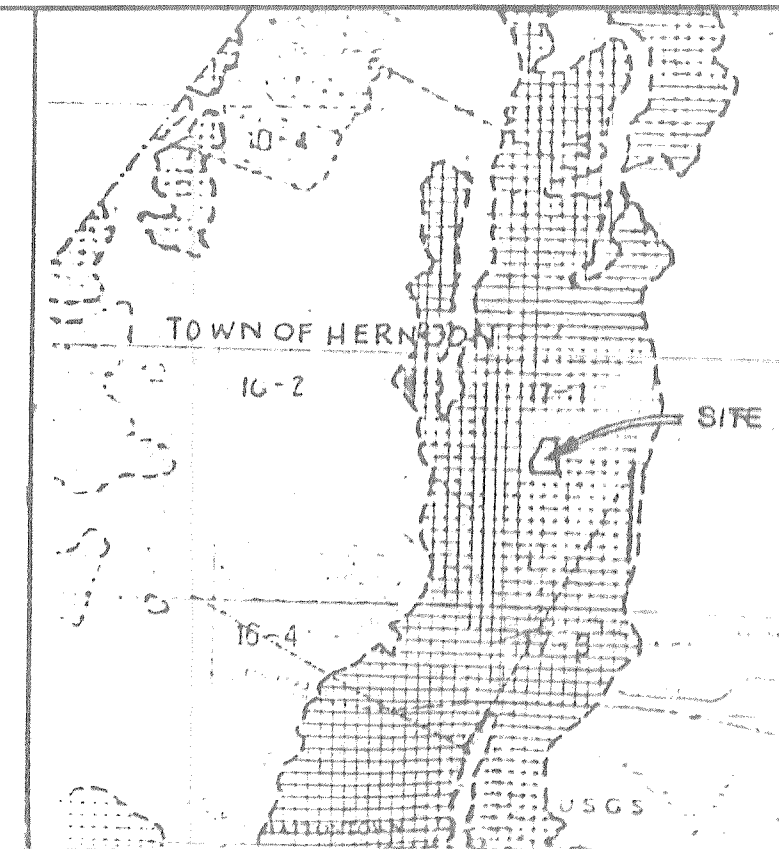
SOIL MAP SCALE 1"=2000'
