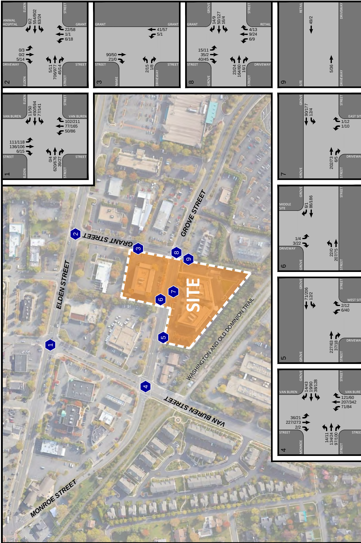
Figure 7 2022 Adjusted Baseline Traffic Volumes
