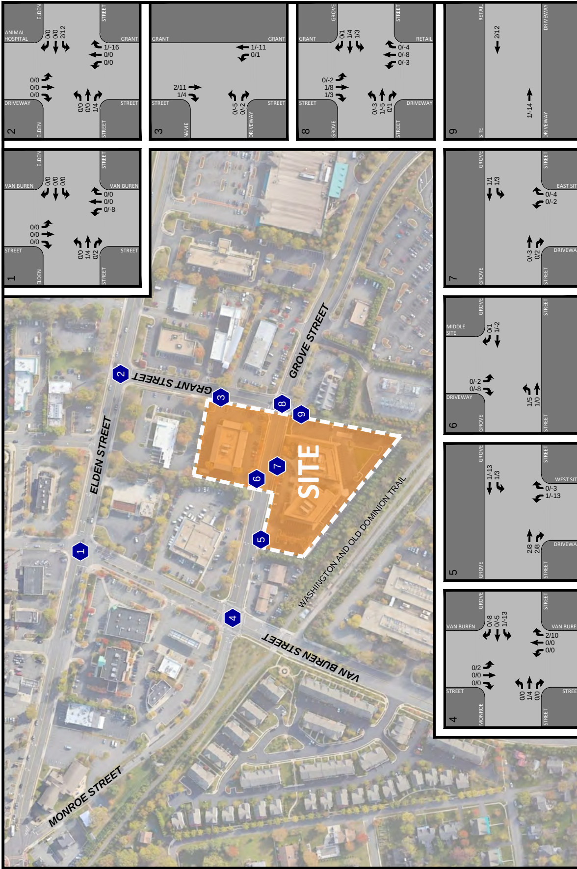
Figure 13 Net Site Generated Trips
