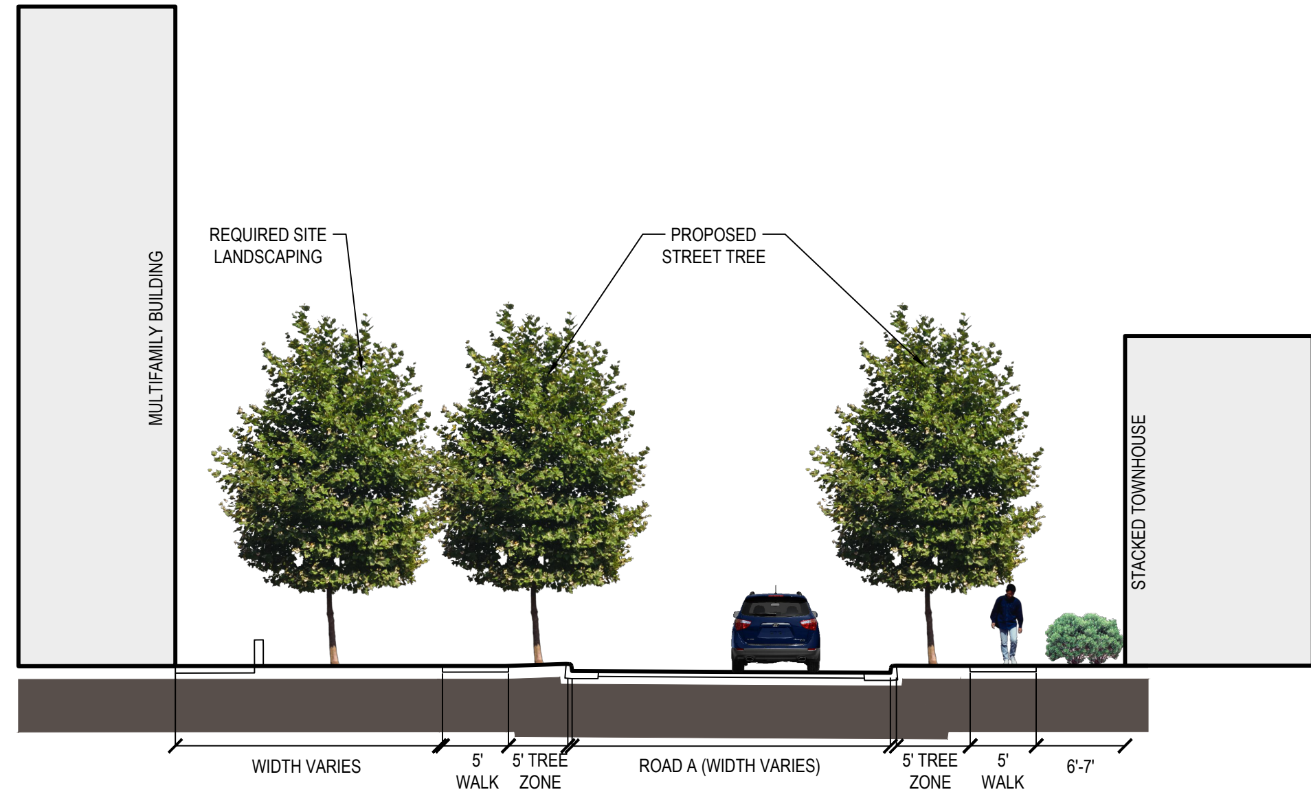
4 ROAD 'A' Scale: 1" = 10'
