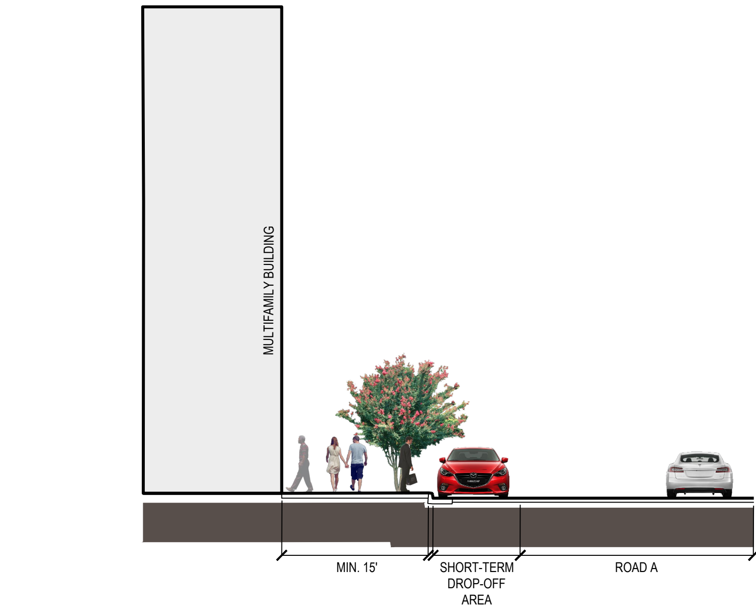
5 MULTIFAMILY DROP-OFF Scale: 1" = 10'
