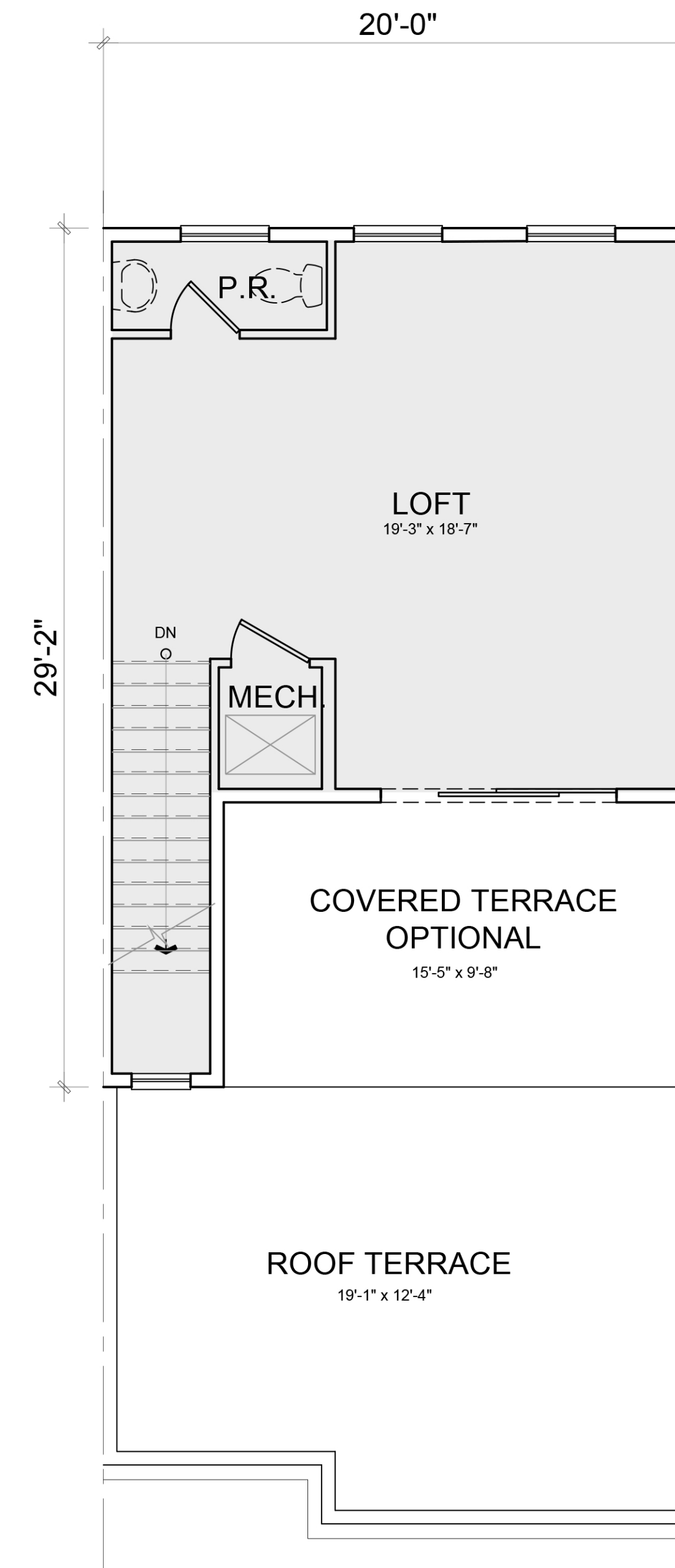
FOURTH FLOOR PLAN AREA: 408 SQ. FT. TOTAL AREA: 2,411 SQ. FT. TOTAL AREA WITH FINISHES: 2,436 SQ. FT.
