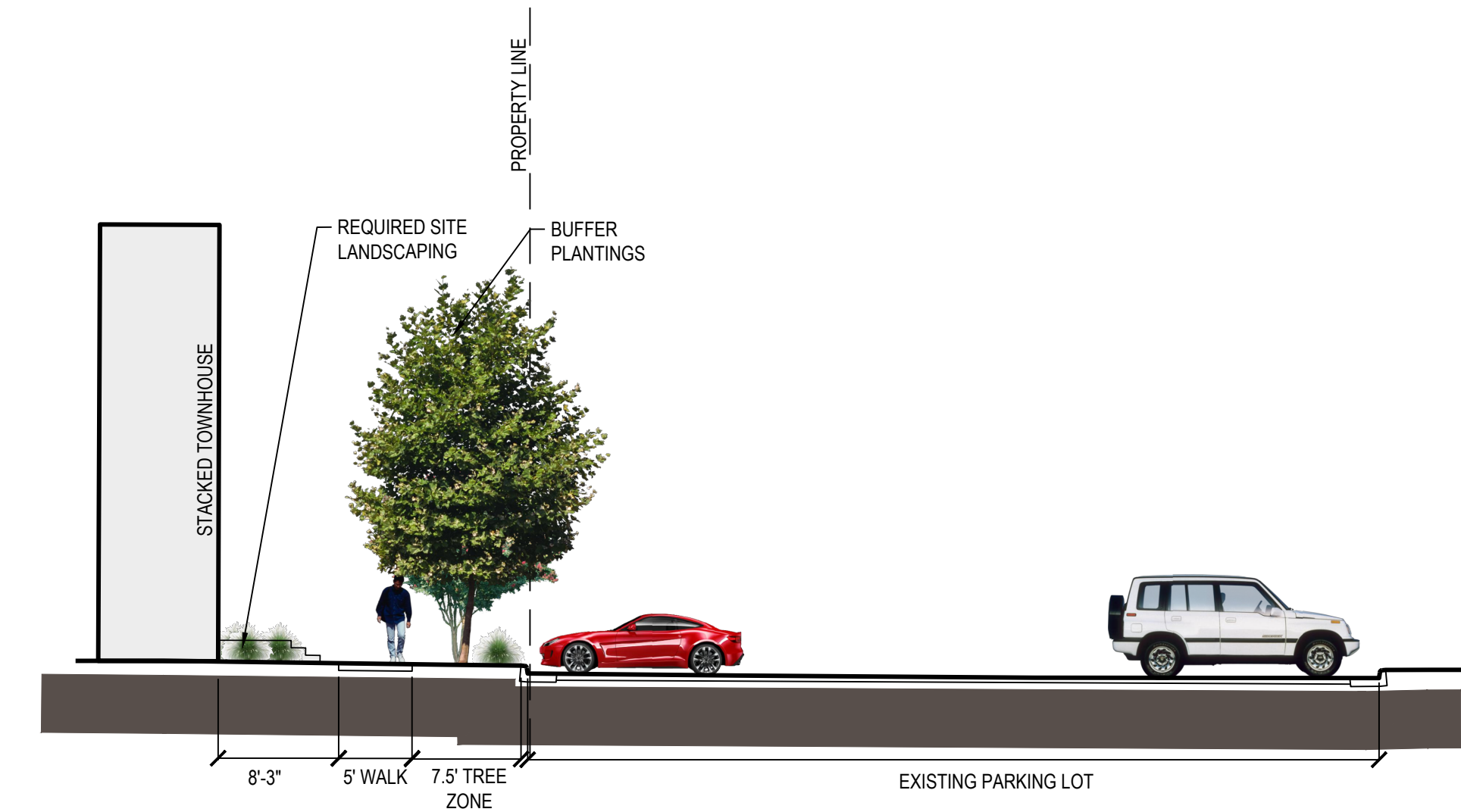
12 LANDSCAPE BUFFER: EAST Scale: 1" = 10'
