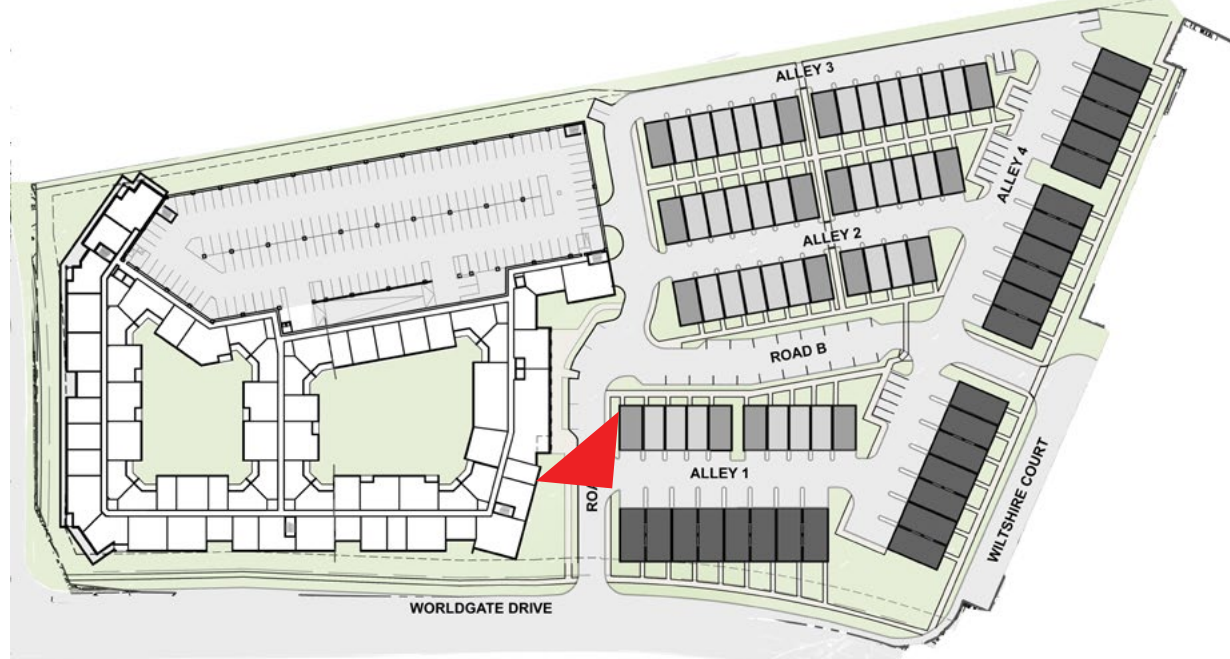
KEY PLAN
