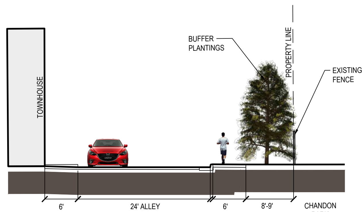
7 LANDSCAPE BUFFER: NORTH Scale: 1" = 10'
