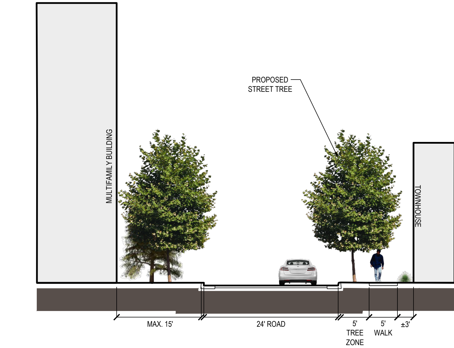
6 ROAD 'A' Scale: 1" = 10'
