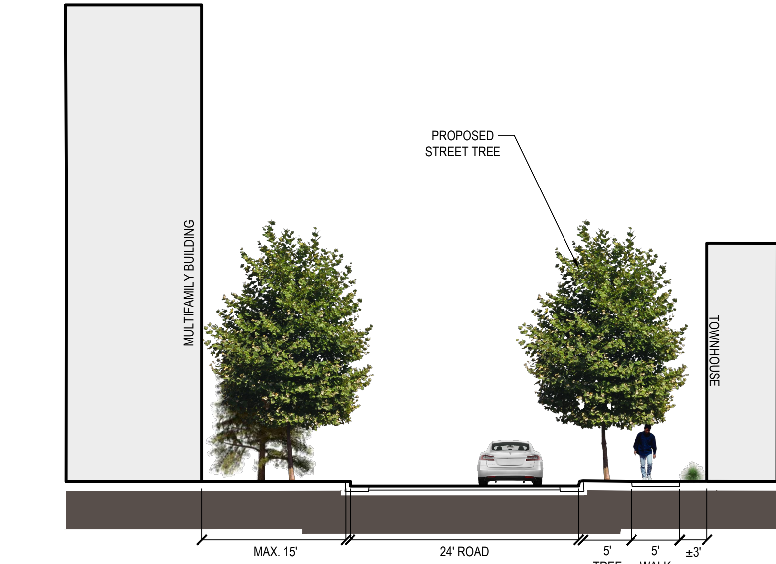
6 ROAD 'A' Scale: 1" = 10'
