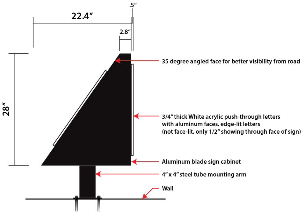
TOP VIEW OF PROPOSED SIGN SHAPE:
